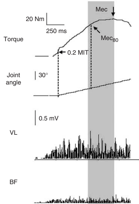
Figure 4 Representative knee extension torque, knee joint angle and rectified EMG data for vastus lateralis (VL) and biceps femoris (BF) performed under eccentric contraction by one of the patients. The first dashed line and arrow show the threshold level necessary to activate the dynamometer servo-motor and initiate the muscle stretch. The second dashed line and arrow indicate the location on the torque-time curve at which eccentric torque (Mec 60 ) was estimated for a knee joint angle of 60 degrees. The third arrow shows the maximum eccentric torque (Mec) produced during the whole eccentric contraction. The 400 ms window (shaded region) was used to determine EMG rms for VL and BF.
