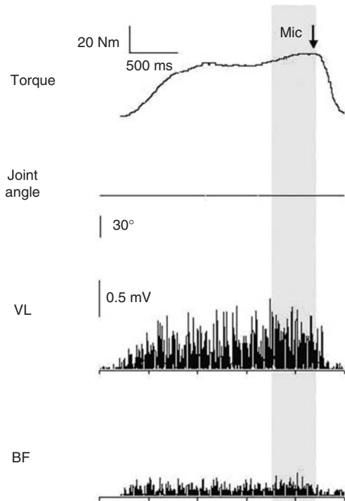
Figure 2 Representative isometric knee extension torque, knee joint angle and rectified EMG data for vastus lateralis (VL) and biceps femoris (BF) performed without time constraint by one of the patients. The arrow indicates the location at which the maximum isometric torque (MIT) was determined. The shaded area represents 400 ms window used for computation of root mean square EMG ( EMG_{rms} ) values for VL and BF.
